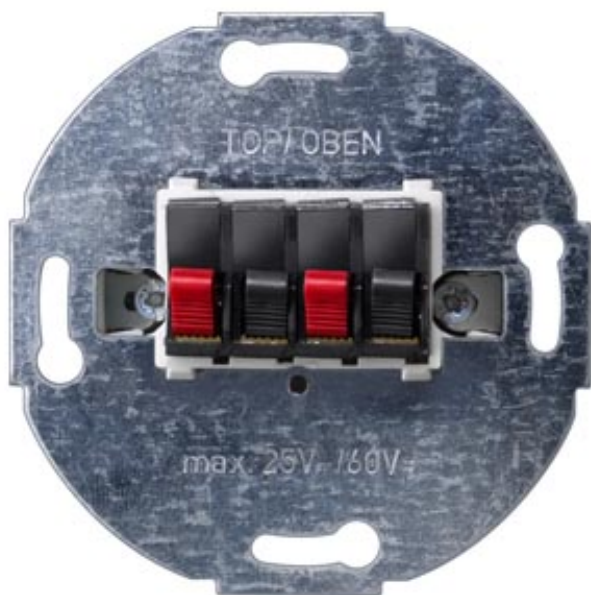
DELTA LOUDSPEAKER OUTLET BOX 2FOLD, AC 25V DC 60V UP TO 10MM2 RELEASE LEVER
